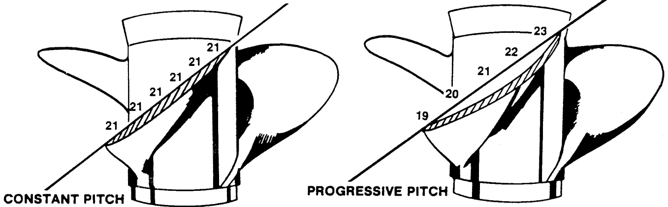
Comparison of a constant and progressive pitch propeller. Notice how the pitch of the progressive pitch propeller, right, changes to give the blade more thrust and therefore, the boat more speed.
