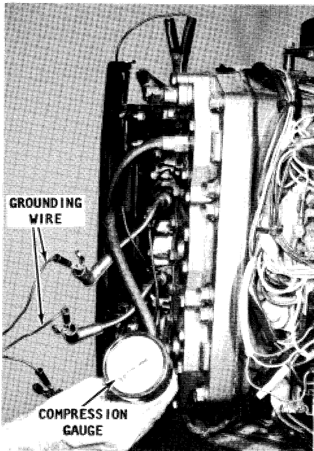
All spark plugs should be "grounded" while making compression tests. This action will prevent placing an extra load on the ignition coil.
