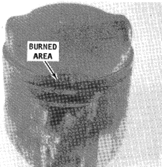
Damaged piston, probably caused by inaccurate fuel mixture, or improper timing.
