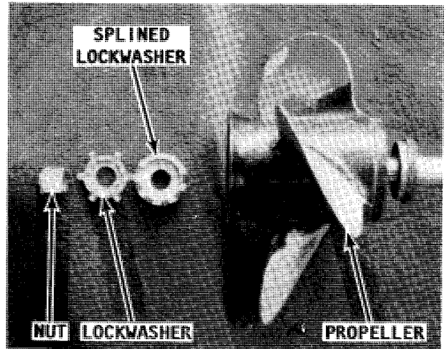
Typical attaching hardware for a propeller.
