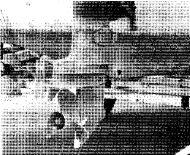
A boat and lower unit covered with marine growth. Such a condition is a serious hinderance to performance and cannot be corrected by tuning the powerhead.
