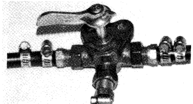
A three-position valve permits fuel to be drawn from either of two tanks or shut off completely. Such an arrangement prevents accidental siphoning of fuel from the tank. The inside diameter of the valve should be at 5/16" (7.94mm).
